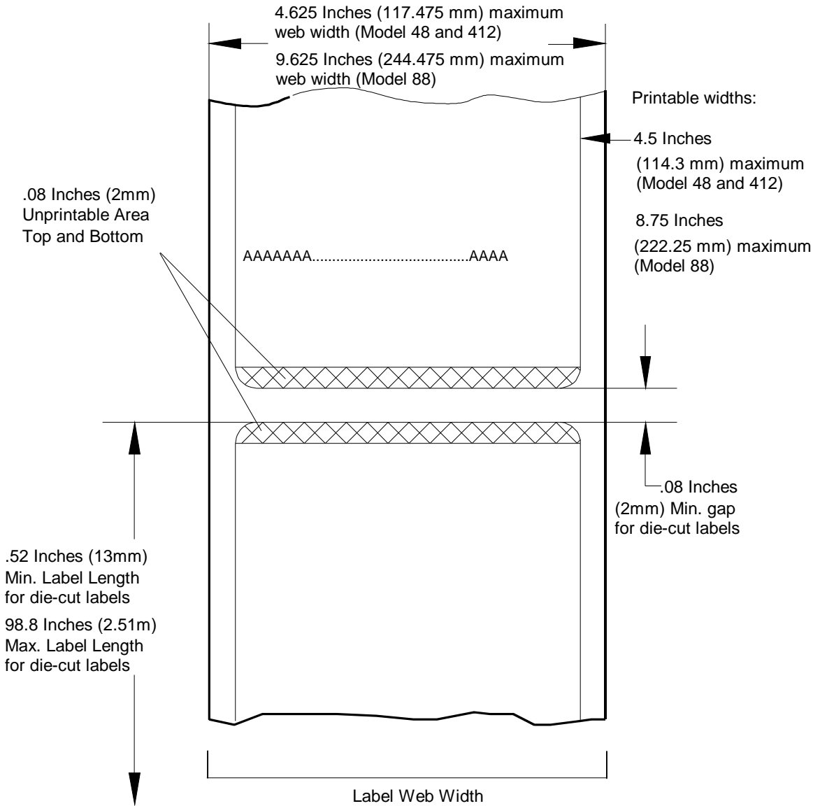
Figure 1-2 Printable Area
